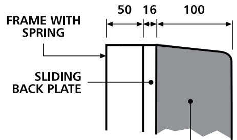
RUBBER BUMPER* (DB3010)
