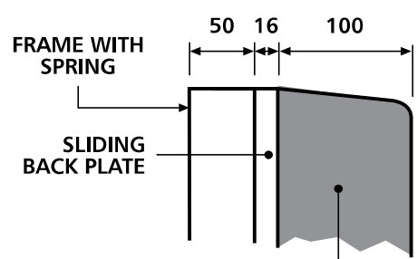
RUBBER BUMPER* (DB1810)
